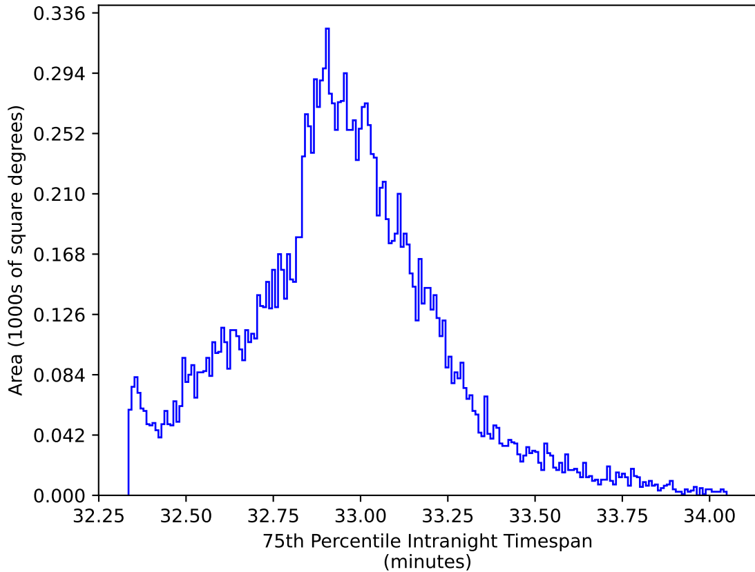
ddf_acor_sf15_lsf20_lsr50_v3.4_10yrs WFD y band: 75th Percentile Intranight Timespan
