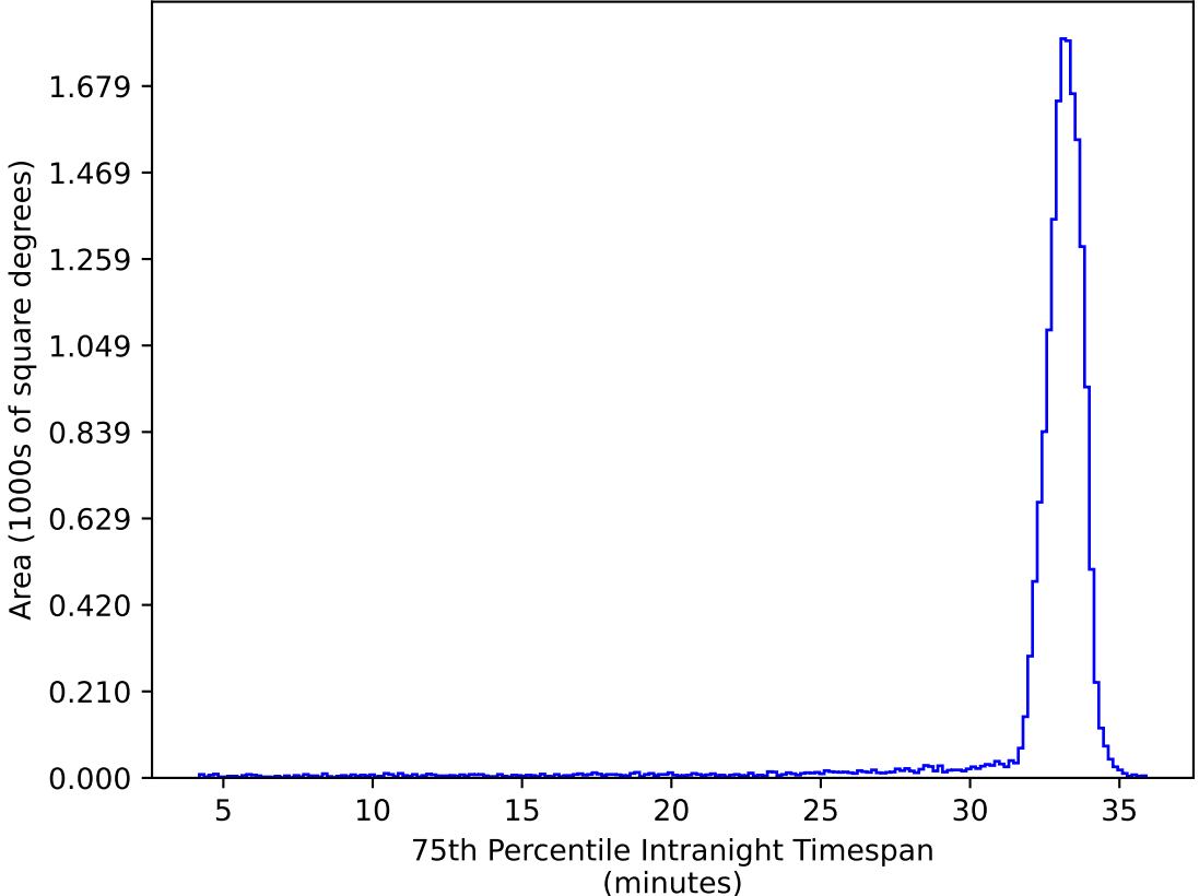
ddf_acor_sf15_lsf20_lsr50_v3.4_10yrs WFD ug bands: 75th Percentile Intranight Timespan
