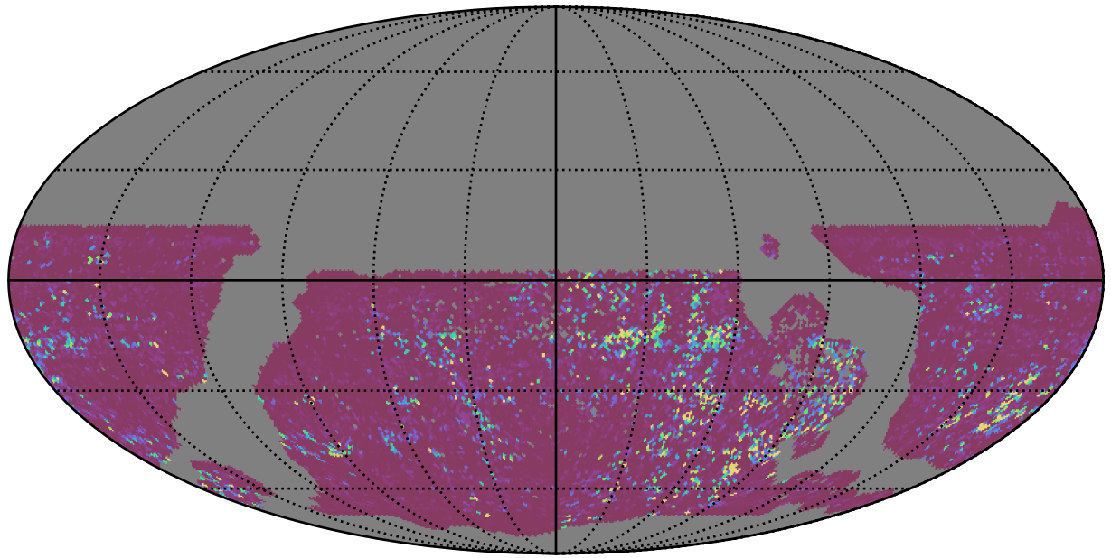
ddf_acor_sf15_lsf20_lsr50_v3.4_10yrs WFD u band: 75th Percentile Intranight Timespan
