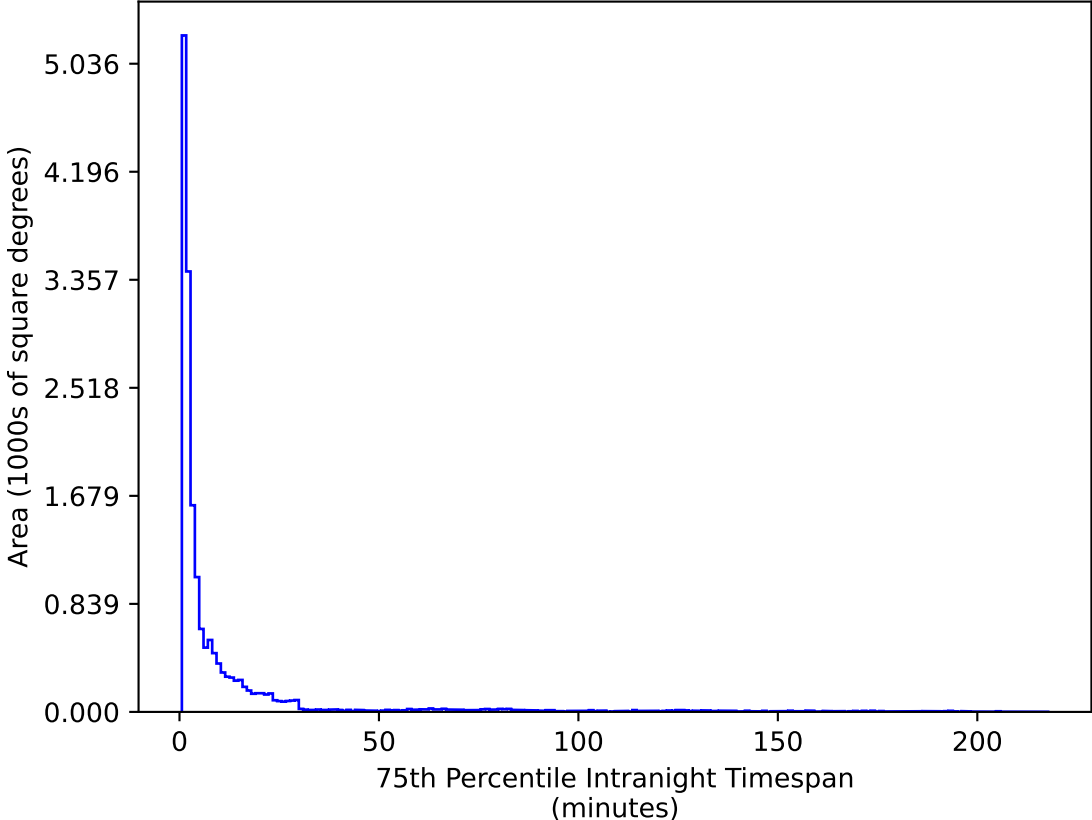
ddf_acor_sf15_lsf20_lsr50_v3.4_10yrs WFD u band: 75th Percentile Intranight Timespan
