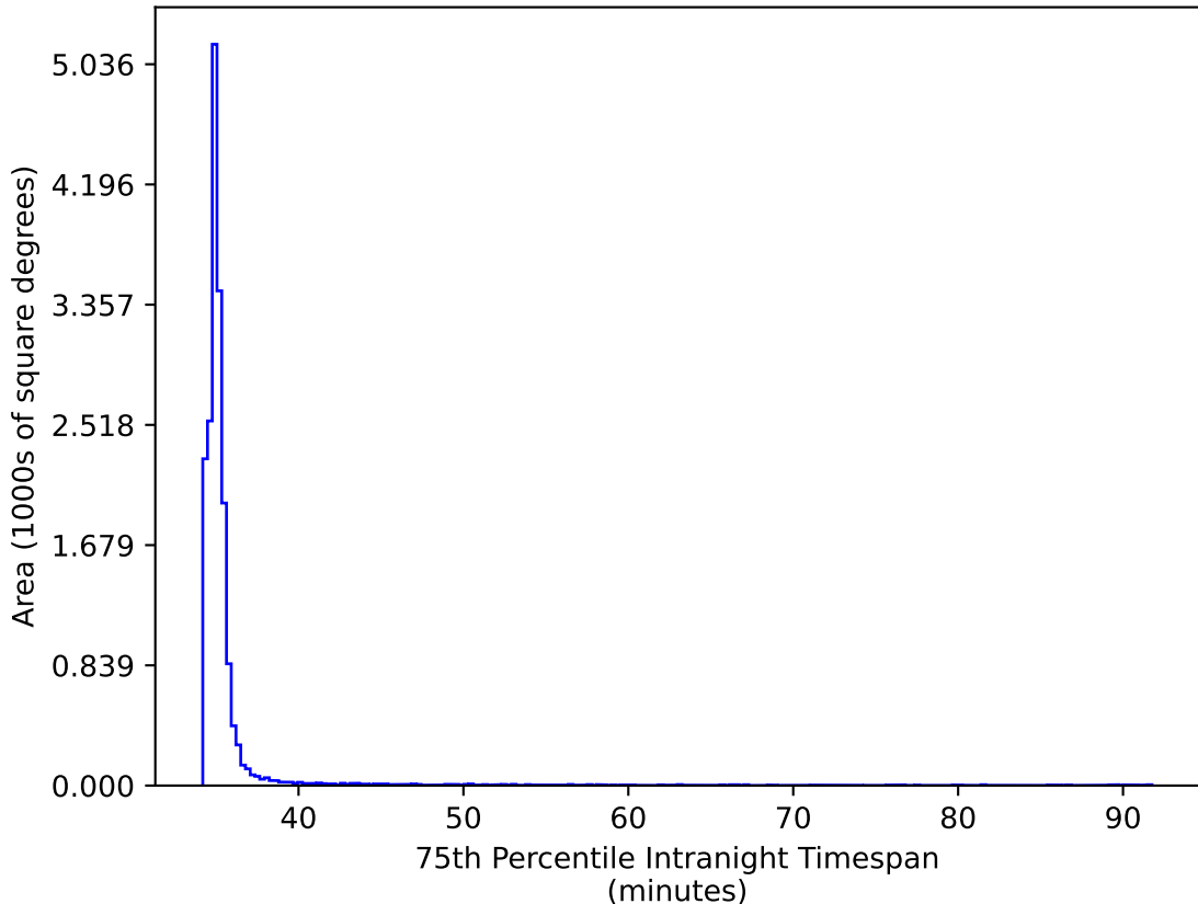
ddf_acor_sf15_lsf20_lsr50_v3.4_10yrs WFD ri bands: 75th Percentile Intranight Timespan
