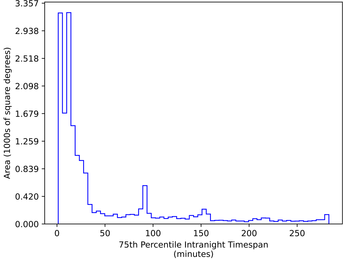
ddf_acor_sf15_ls20_lsr50_v3.4_10yrs WFD r band: 75th Percentile Intranight Timespan
