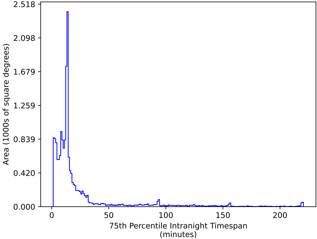
ddf_acor_sf15_ls20_lsr50_v3.4_10yrs WFD i band: 75th Percentile Intranight Timespan
