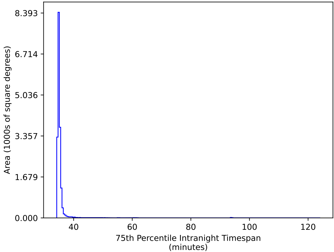
ddf_acor_sf15_lsf20_lsr50_v3.4_10yrs WFD gr bands: 75th Percentile Intranight Timespan
