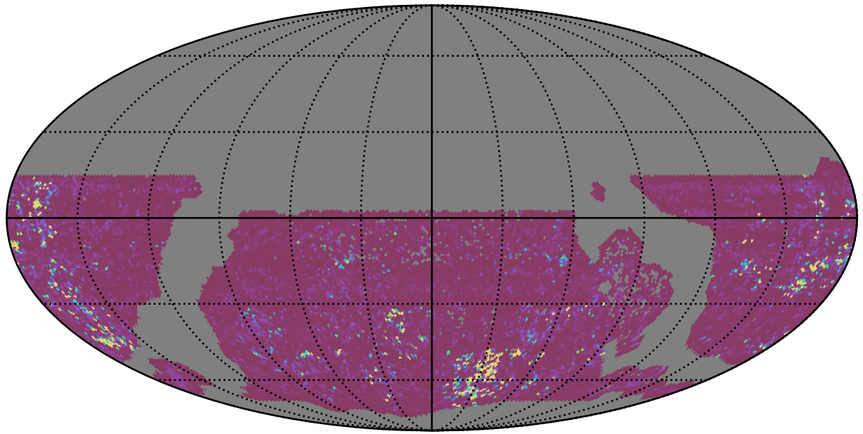
ddf_acor_sf15_lsf20_lsr50_v3.4_10yrs WFD g band: 75th Percentile Intranight Timespan
