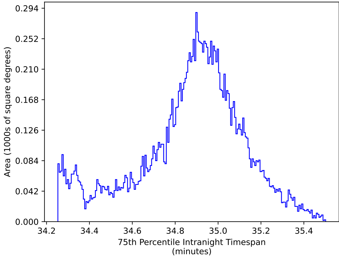
ddf_acor_sf15_lsf20_lsr50_v3.4_10yrs WFD: 75th Percentile Intranight Timespan
