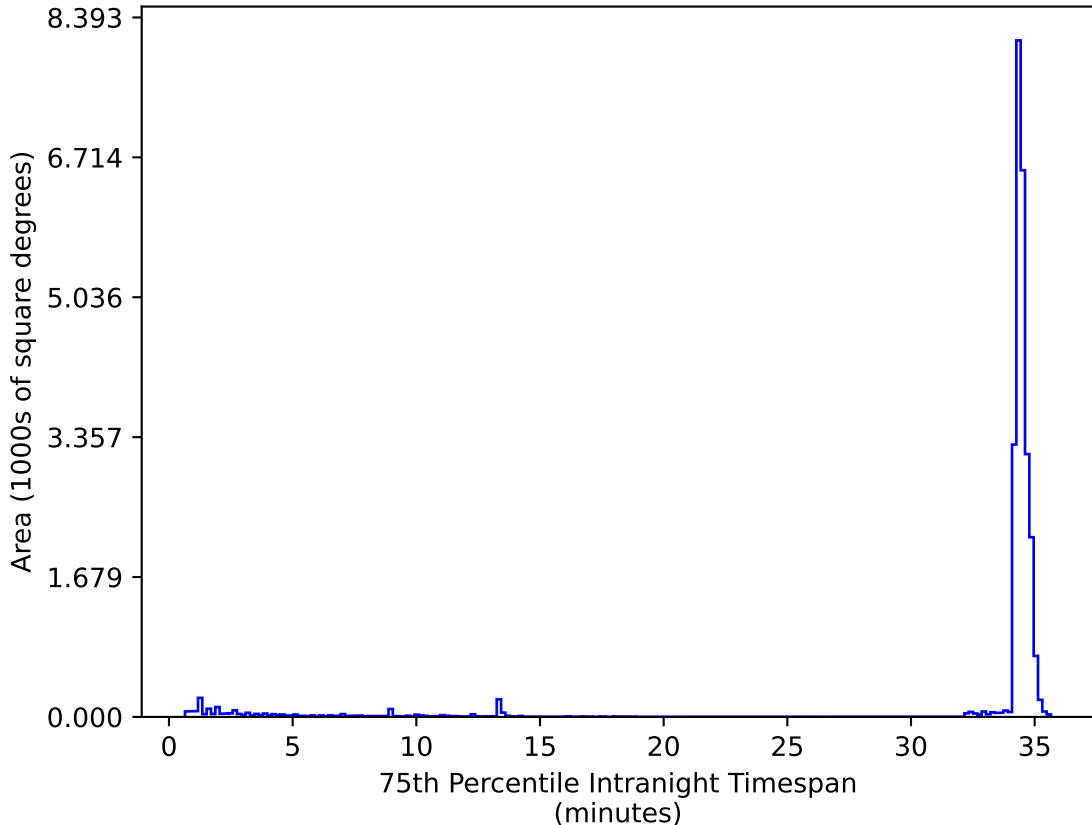
ddf_acor_sf15_lsf20_lsr50_v3.4_10yrs All sky zy bands: 75th Percentile Intranight Timespan
