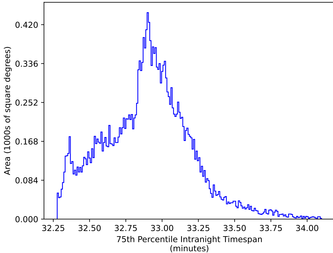
ddf_acor_sf15_lsf20_lsr50_v3.4_10yrs All sky y band: 75th Percentile Intranight Timespan
