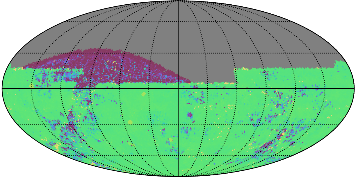
ddf_acor_sf15_lsf20_lsr50_v3.4_10yrs All sky ug bands: 75th Percentile Intranight Timespan
