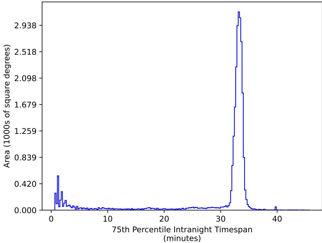
ddf_acor_sf15_lsf20_lsr50_v3.4_10yrs All sky ug bands: 75th Percentile Intranight Timespan
