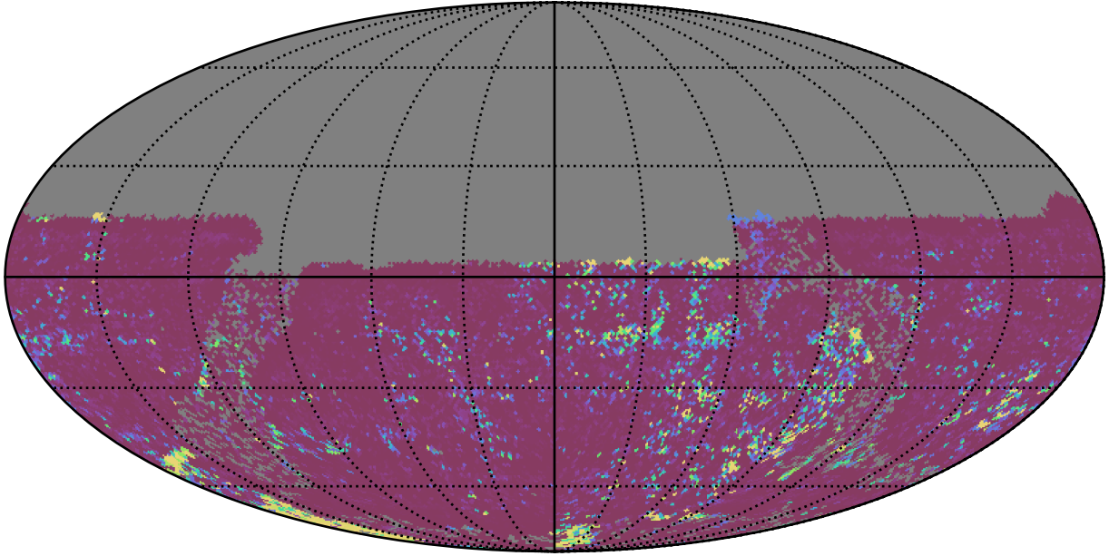
ddf_acor_sf15_lsf20_lsr50_v3.4_10yrs All sky u band: 75th Percentile Intranight Timespan
