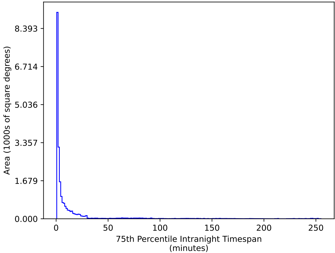
ddf_acor_sf15_lsf20_lsr50_v3.4_10yrs All sky u band: 75th Percentile Intranight Timespan
