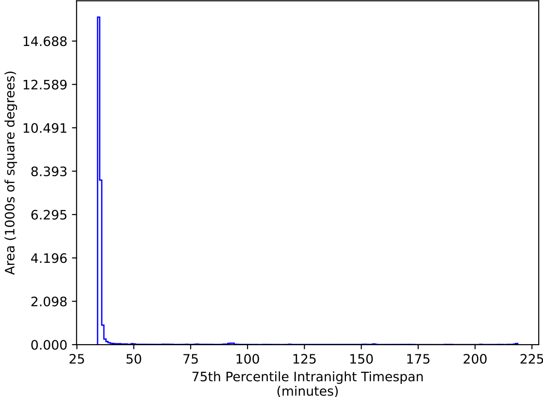
ddf_acor_sf15_lsf20_lsr50_v3.4_10yrs All sky ri bands: 75th Percentile Intranight Timespan
