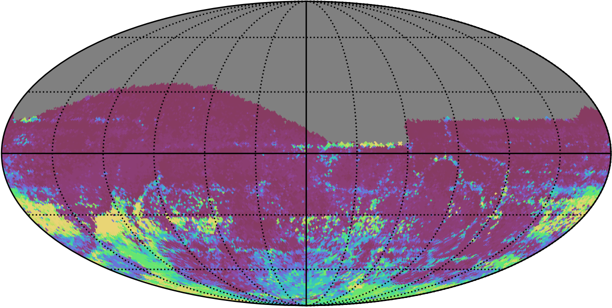
ddf_acor_sf15_lsf20_lsr50_v3.4_10yrs All sky r band: 75th Percentile Intranight Timespan
