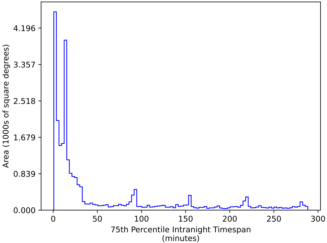
ddf_acor_sf15_ls20_lsr50_v3.4_10yrs All sky r band: 75th Percentile Intranight Timespan
