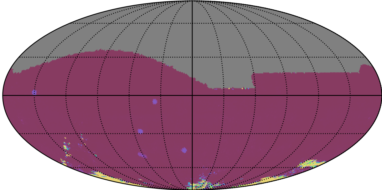
ddf_acor_sf15_lsf20_lsr50_v3.4_10yrs All sky iz bands: 75th Percentile Intranight Timespan
