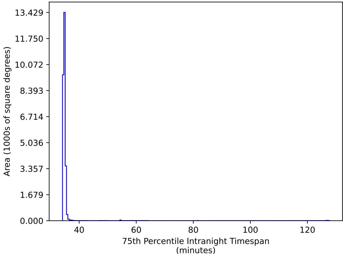
ddf_acor_sf15_lsf20_lsr50_v3.4_10yrs All sky iz bands: 75th Percentile Intranight Timespan
