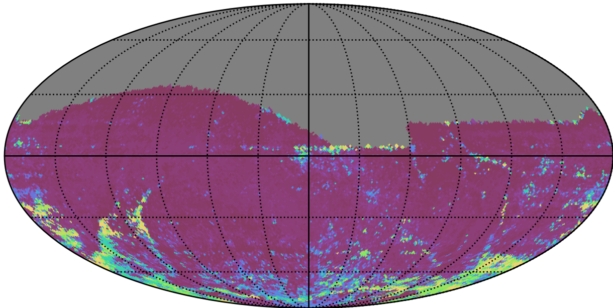
ddf_acor_sf15_lsf20_lsr50_v3.4_10yrs All sky i band: 75th Percentile Intranight Timespan
