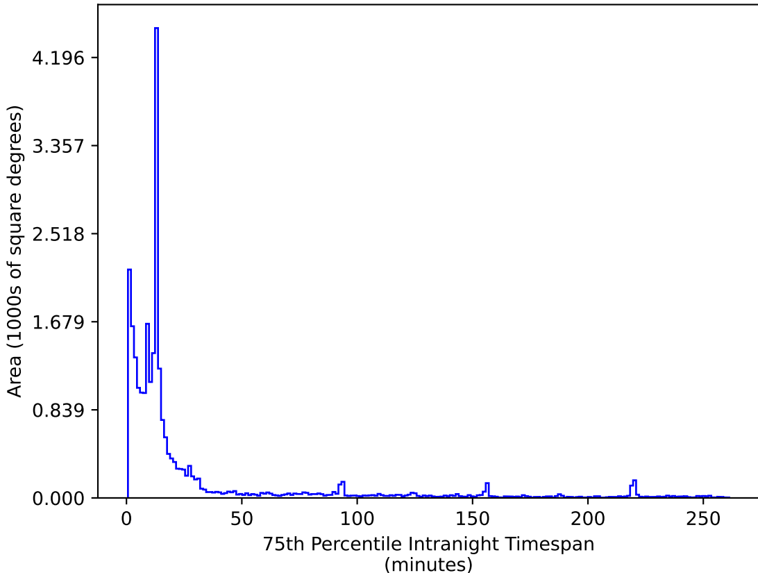
ddf_acor_sf15_lsf20_lsr50_v3.4_10yrs All sky i band: 75th Percentile Intranight Timespan
