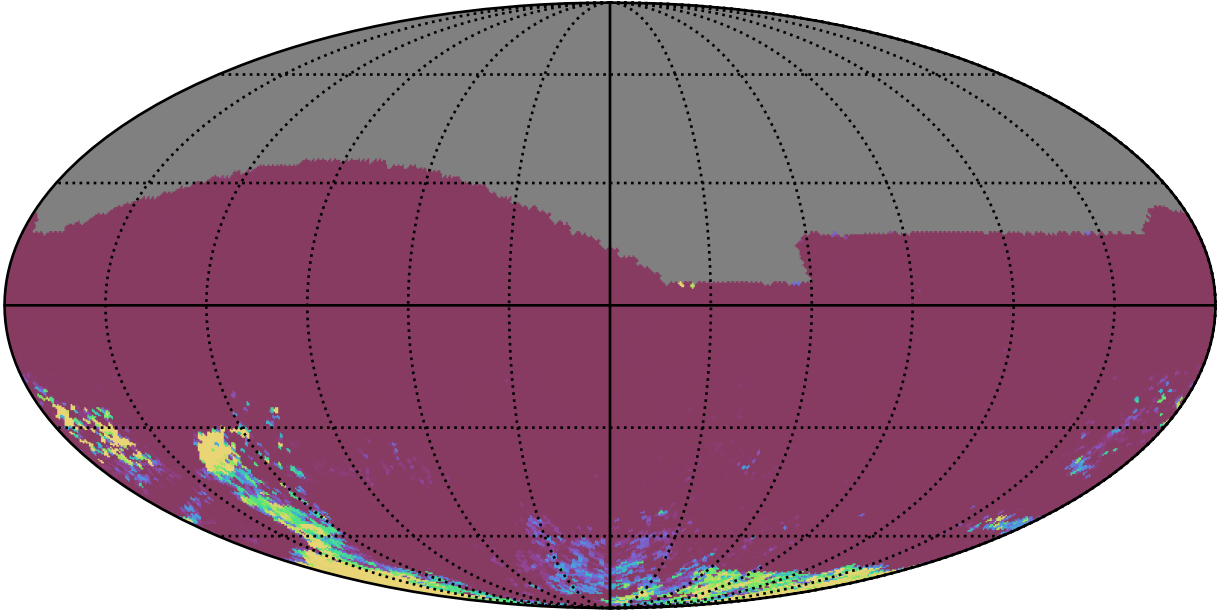
ddf_acor_sf15_lsf20_lsr50_v3.4_10yrs All sky gr bands: 75th Percentile Intranight Timespan
