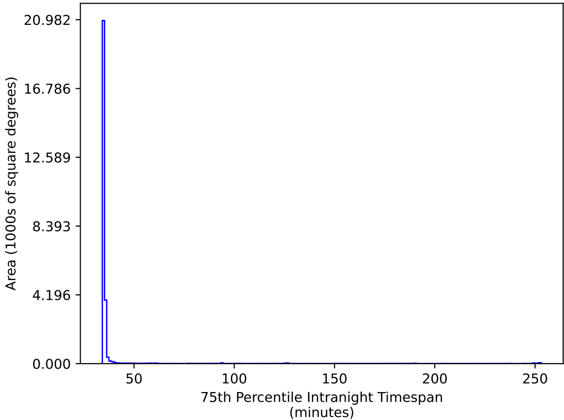
ddf_acor_sf15_lsf20_lsr50_v3.4_10yrs All sky gr bands: 75th Percentile Intranight Timespan
