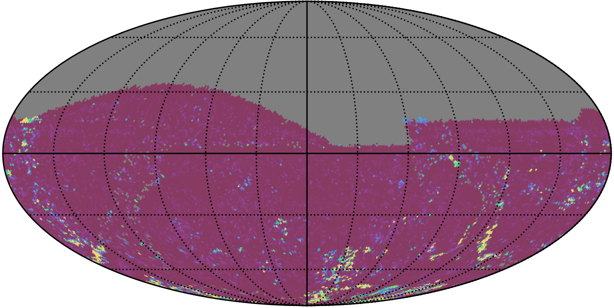
ddf_acor_sf15_lsf20_lsr50_v3.4_10yrs All sky g band: 75th Percentile Intranight Timespan
