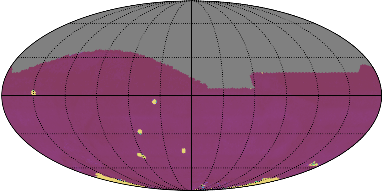
ddf_acor_sf15_lsf20_lsr50_v3.4_10yrs All sky all bands: 75th Percentile Intranight Timespan
