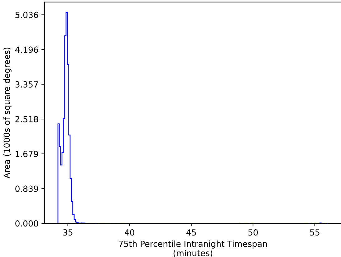
ddf_acor_sf15_lsf20_lsr50_v3.4_10yrs All sky all bands: 75th Percentile Intranight Timespan
