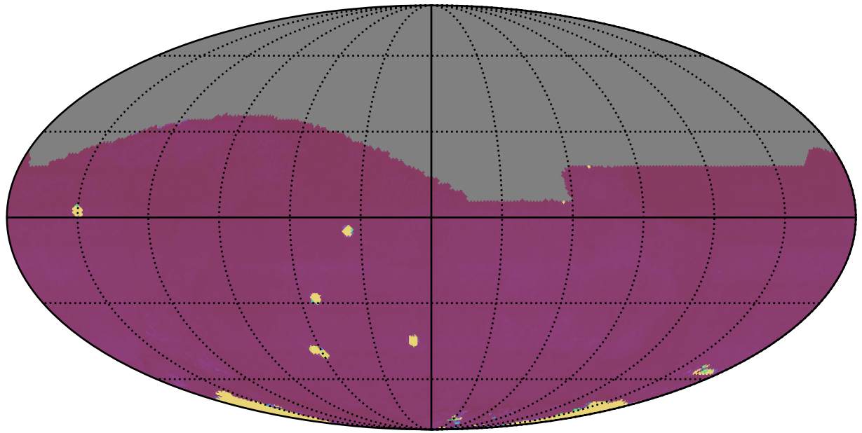
ddf_acor_sf15_lsf20_lsr50_v3.4_10yrs All sky: 75th Percentile Intranight Timespan
