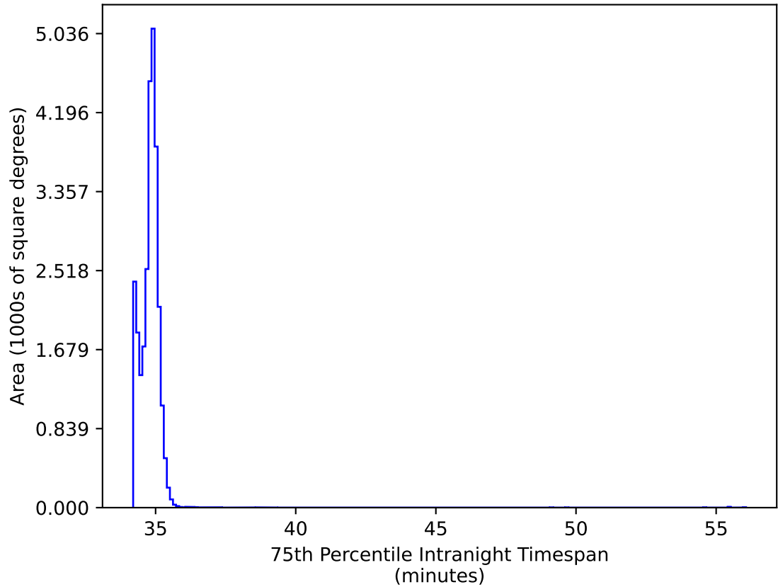
ddf_acor_sf15_lsf20_lsr50_v3.4_10yrs All sky: 75th Percentile Intranight Timespan
