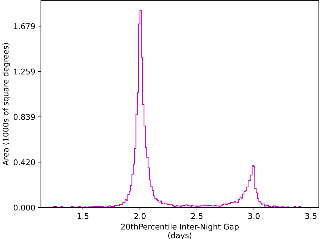
ddf_acor_sf15_lsf20_lsr50_v3.4_10yrs WFD z band: 20thPercentile Inter-Night Gap
