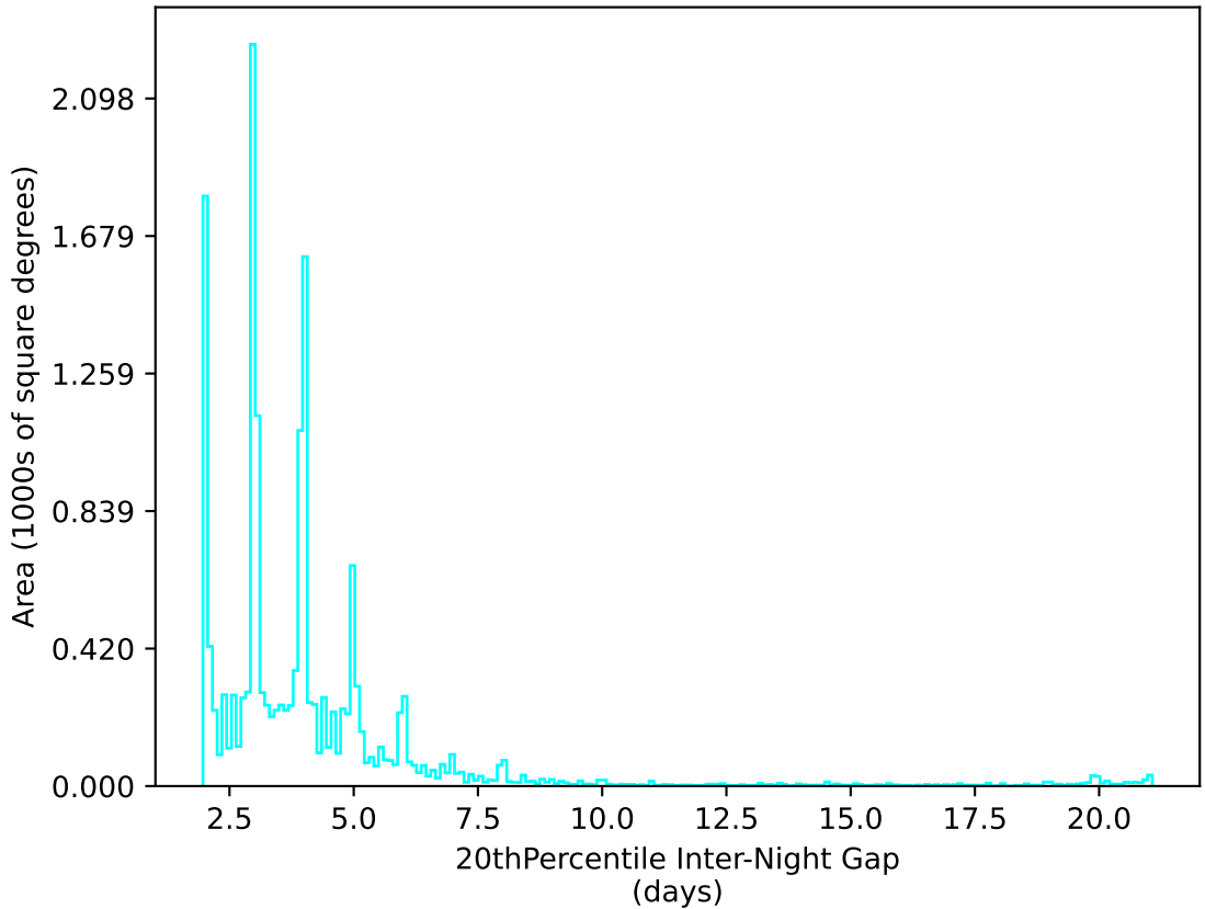
ddf_acor_sf15_lsf20_lsr50_v3.4_10yrs WFD u band: 20thPercentile Inter-Night Gap
