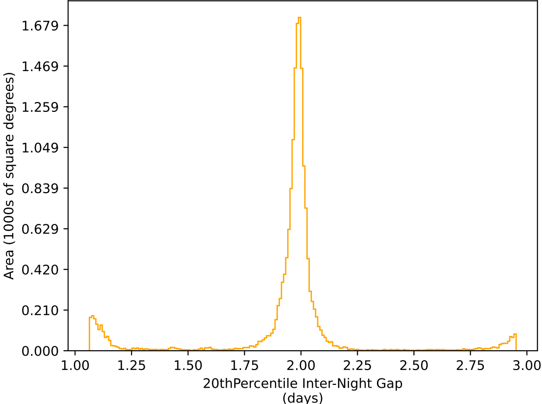
ddf_acor_sf15_lsf20_lsr50_v3.4_10yrs WFD r band: 20thPercentile Inter-Night Gap
