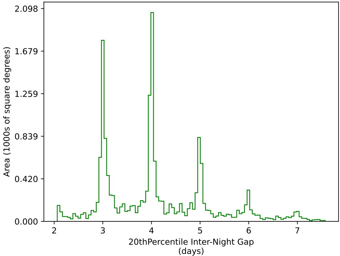
ddf_acor_sf15_lsf20_lsr50_v3.4_10yrs WFD g band: 20thPercentile Inter-Night Gap
