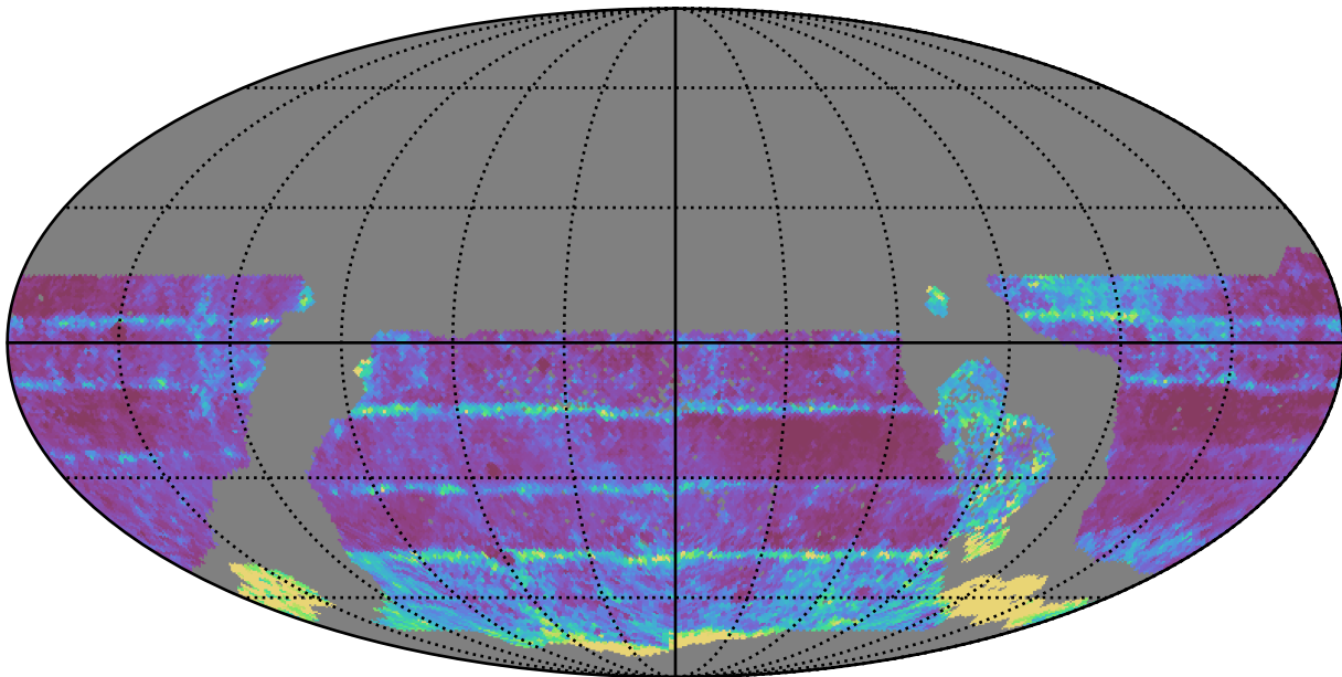
ddf_acor_sf15_lsf20_lsr50_v3.4_10yrs WFD all bands: 20thPercentile Inter-Night Gap
