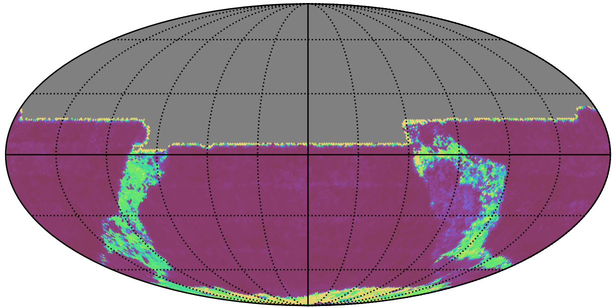
ddf_acor_sf15_lsf20_lsr50_v3.4_10yrs All sky y band: 20thPercentile Inter-Night Gap
