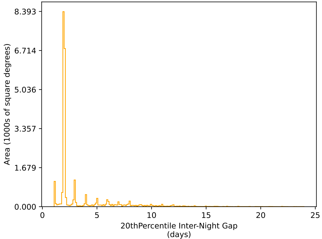
ddf_acor_sf15_lsf20_lsr50_v3.4_10yrs All sky r band: 20thPercentile Inter-Night Gap
