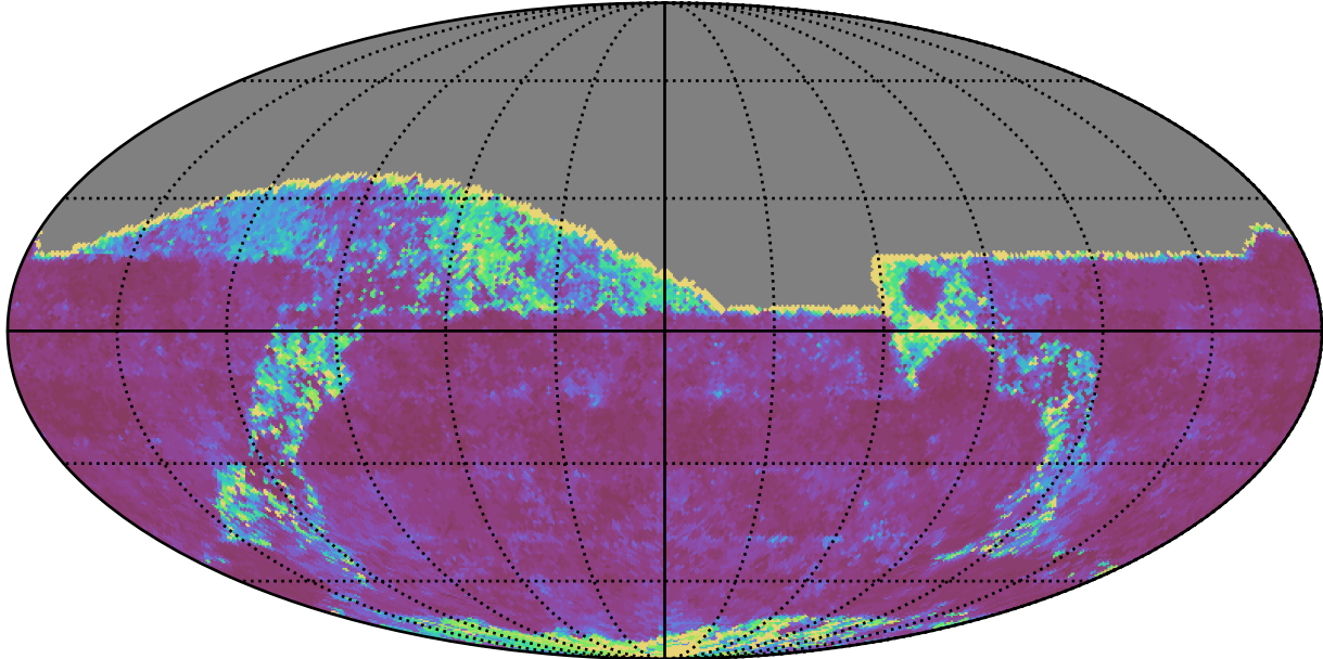
ddf_acor_sf15_lsf20_lsr50_v3.4_10yrs All sky g band: 20thPercentile Inter-Night Gap
