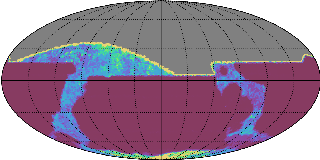
ddf_acor_sf15_lsf20_lsr50_v3.4_10yrs All sky all bands: 20thPercentile Inter-Night Gap
