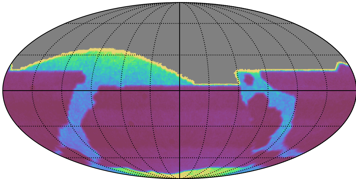
ddf_acor_sf15_lsf20_lsr50_v3.4_10yrs : properMotion
