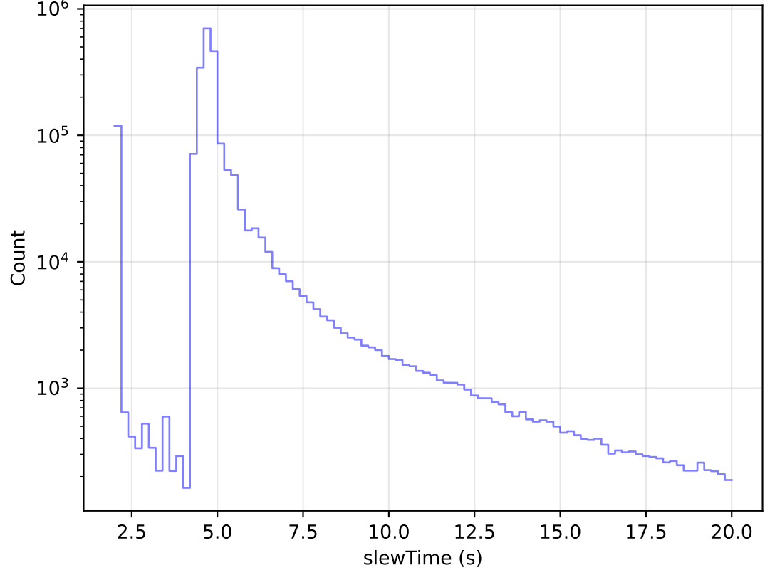
ddf_acor_sf15_Isf20_Isr50_v3.4_10yrs All visits: Zoom Slew Time Histogram
