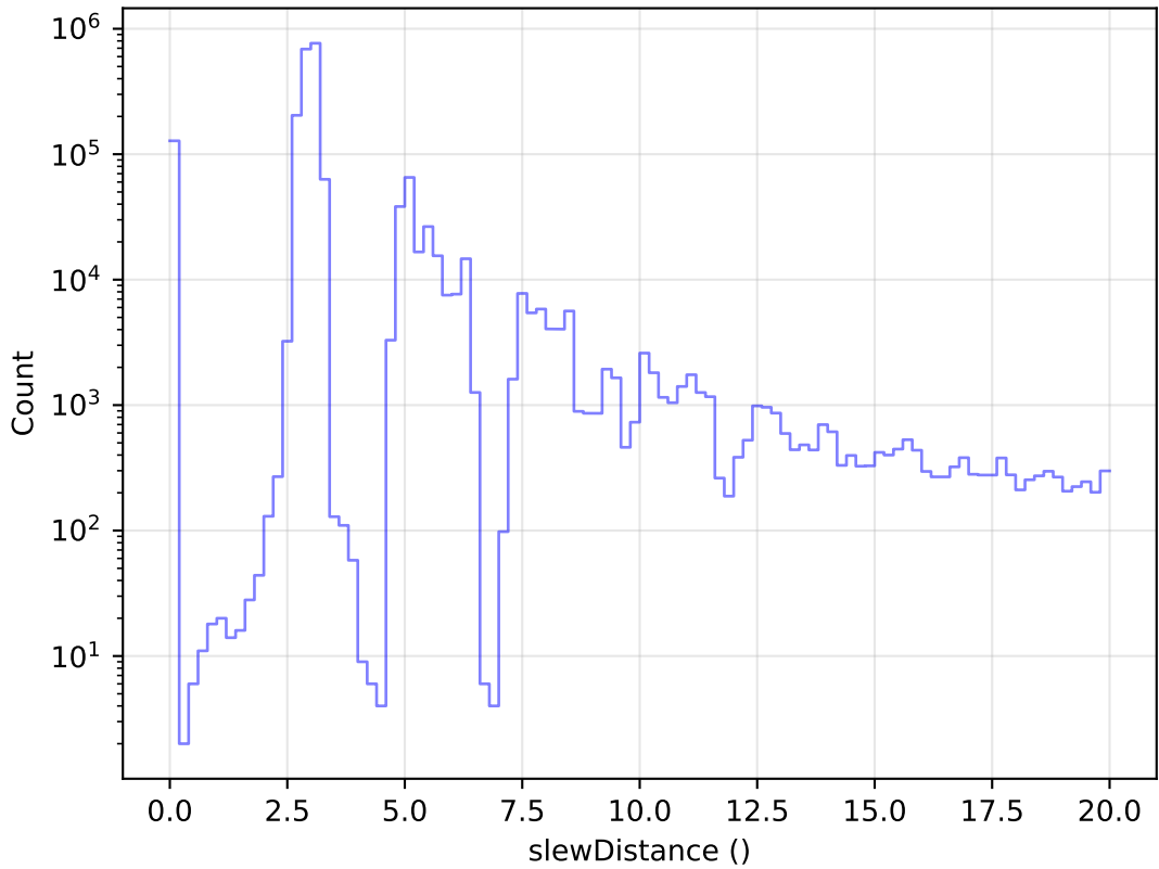
ddf_acor_sf15_lsf20_lsr50_v3.4_10yrs All visits: Zoom Slew Distance Histogram
