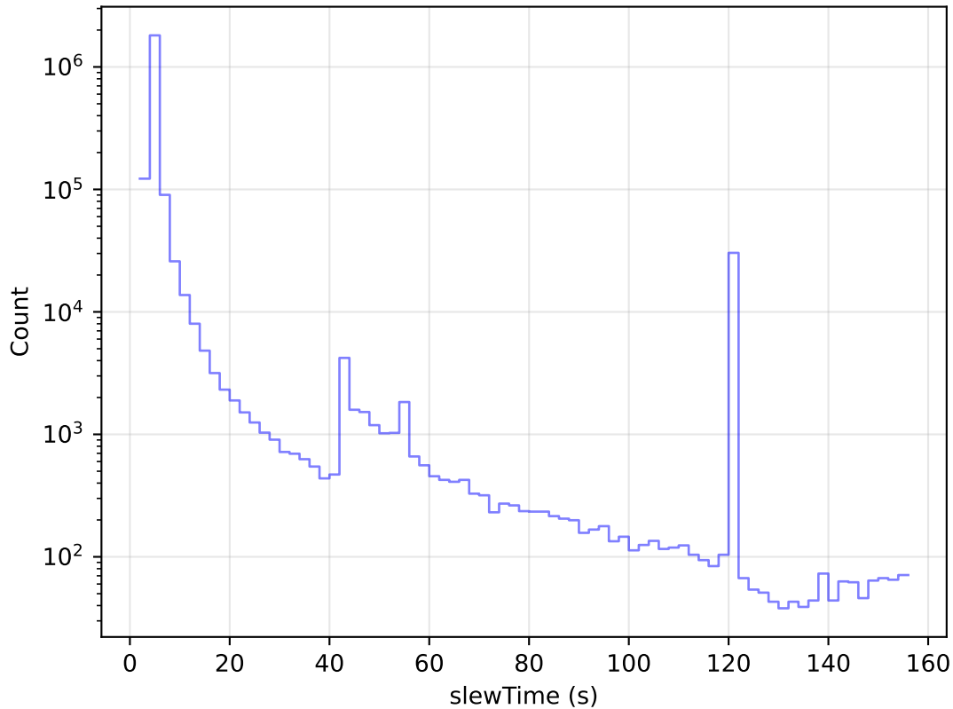
ddf_acor_sf15_lsf20_lsr50_v3.4_10yrs All visits: Slew Time Histogram
