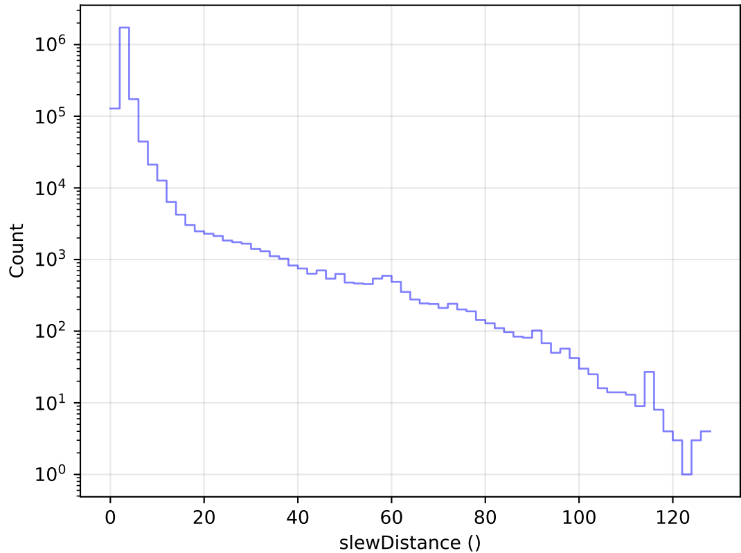
ddf_acor_sf15_lsf20_lsr50_v3.4_10yrs All visits: Slew Distance Histogram
