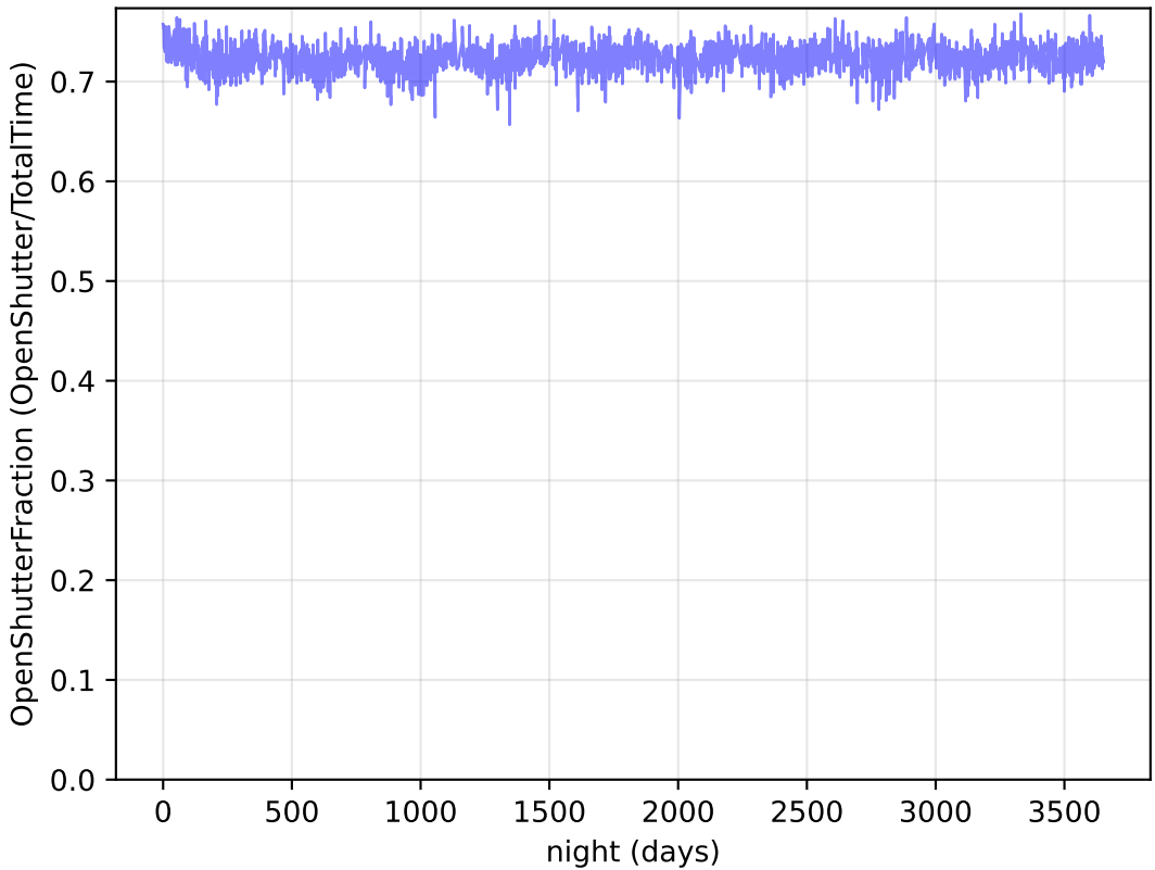
ddf_acor_sf15_lsf20_lsr50_v3.4_10yrs : OpenShutterFraction
