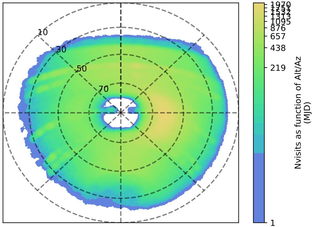
ddf_acor_sf15_lsf20_lsr50_v3.4_10yrs y: Nvisits as function of Alt/Az
