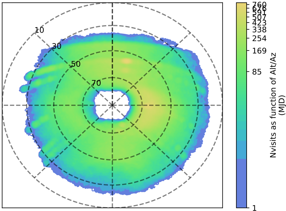
ddf_acor_sf15_lsf20_lsr50_v3.4_10yrs u: Nvisits as function of Alt/Az
