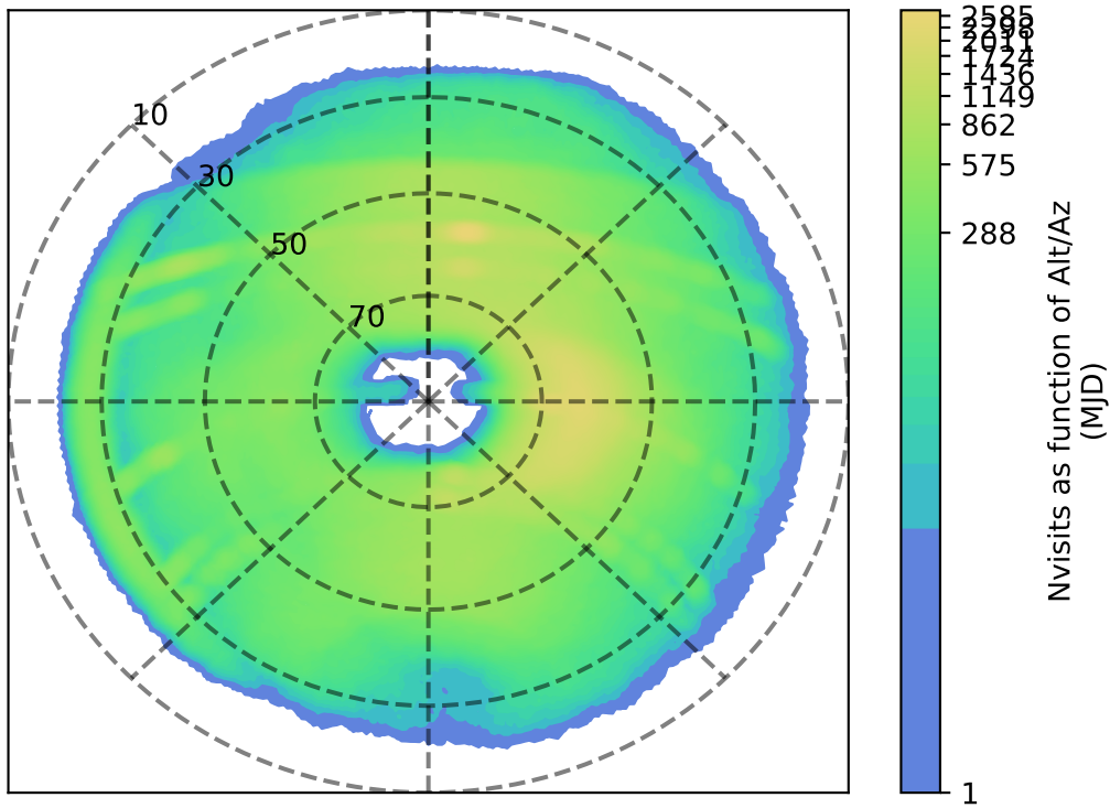
ddf_acor_sf15_ls20_lsr50_v3.4_10yrs r: Nvisits as function of Alt/Az
