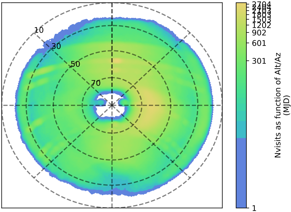
ddf_acor_sf15_ls20_lsr50_v3.4_10yrs i: Nvisits as function of Alt/Az
