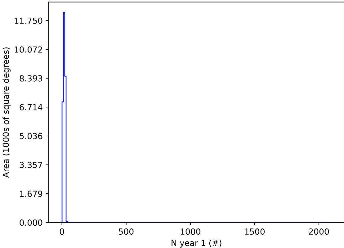
ddf_acor_sf15_lsf20_lsr50_v3.4_10yrs i and night < 365: N year 1
